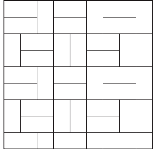
Basket Weave Variation Avenue, Classic
